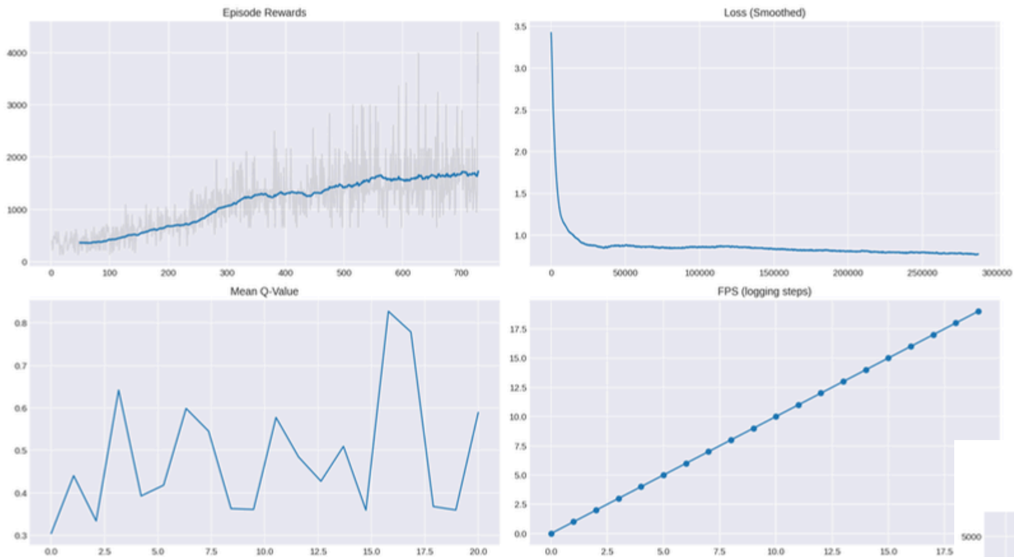
C51 Metrics – BeamRider (Gamma = 0.9)
