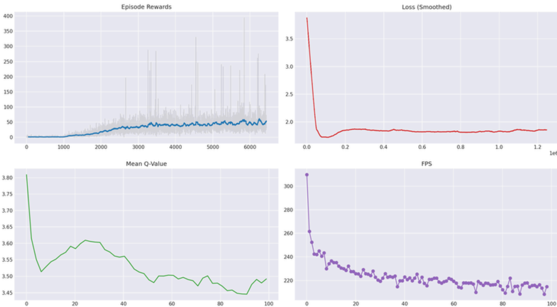
C51 Metrics - 1_Baseline
