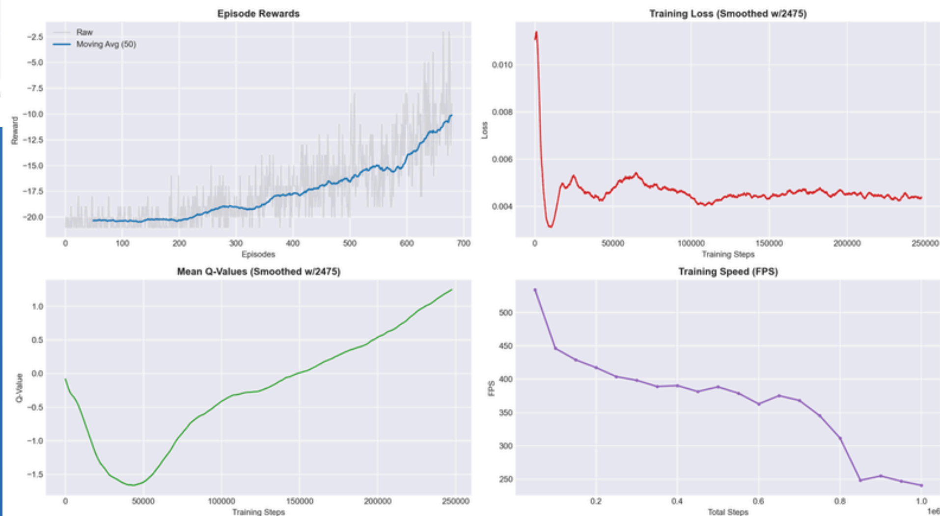
DQN Training Metrics (Decay=500000): PongNoFrameskip-v4
