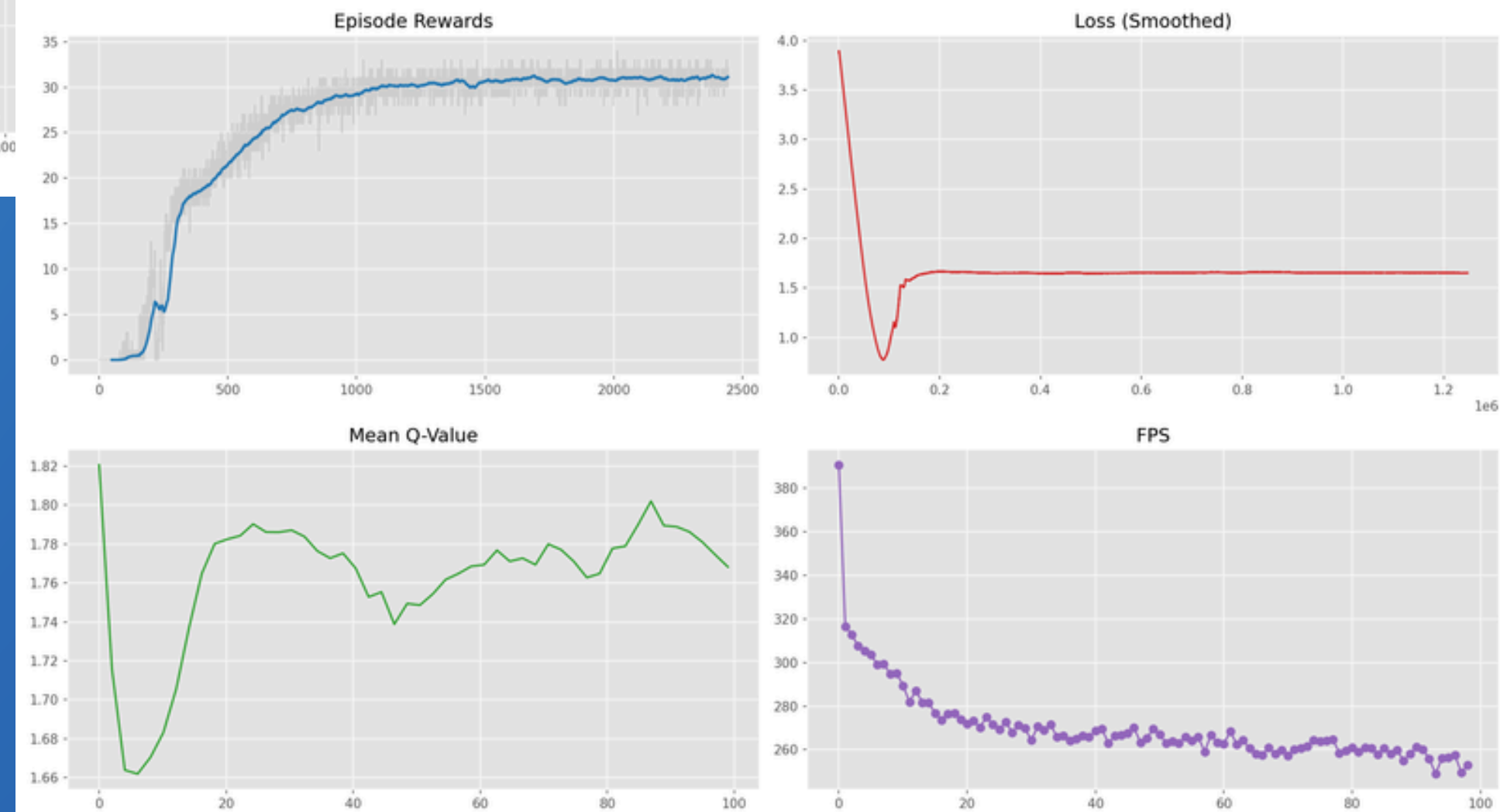
C51 Metrics - 4_Batch_128
