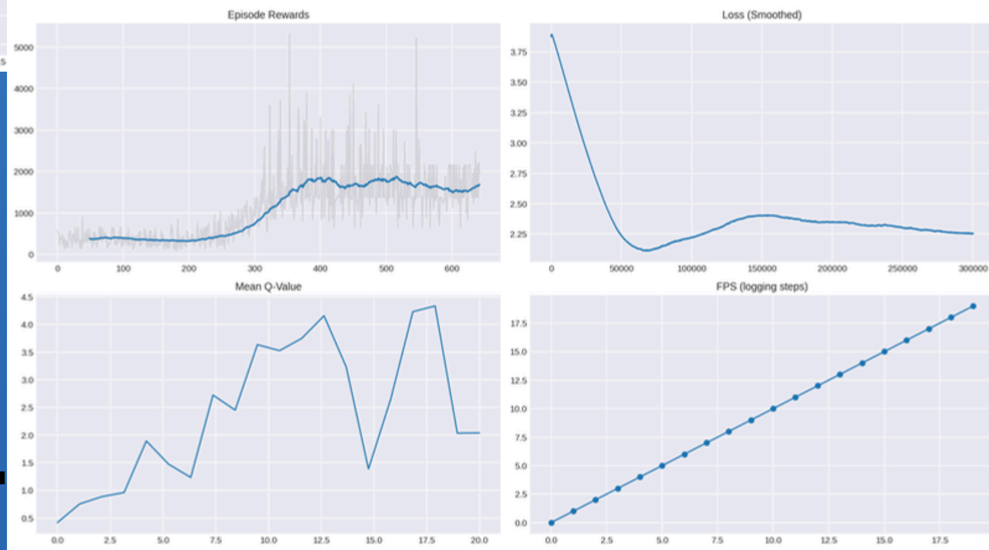
C51 Metrics – BeamRider (LR = 1e-4 )
