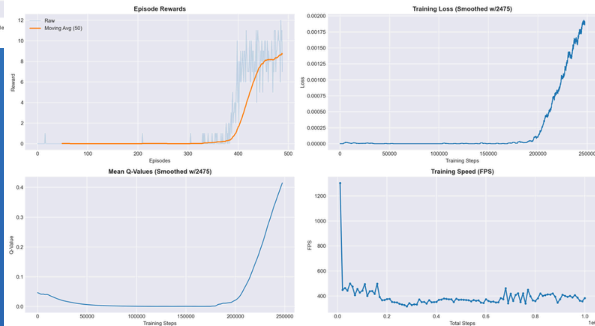
DQN Training Metrics: FreewayNoFrameskip-v4 (Duration: 0:43:27)
