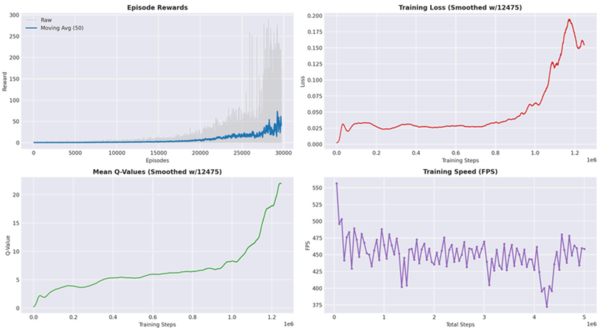
DQN Training Metrics: BreakoutNoFrameskip-v4
