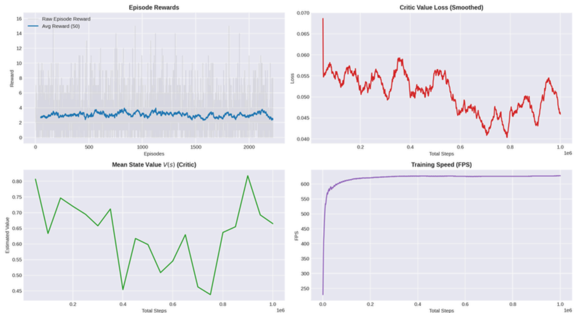
PPO Training Metrics: BeamRiderNoFrameskip-v4
