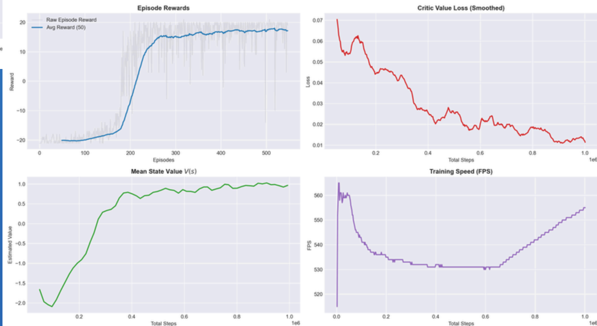
PPO Metrics (LR=0.00025, BS=64): PongNoFrameskip-v4
