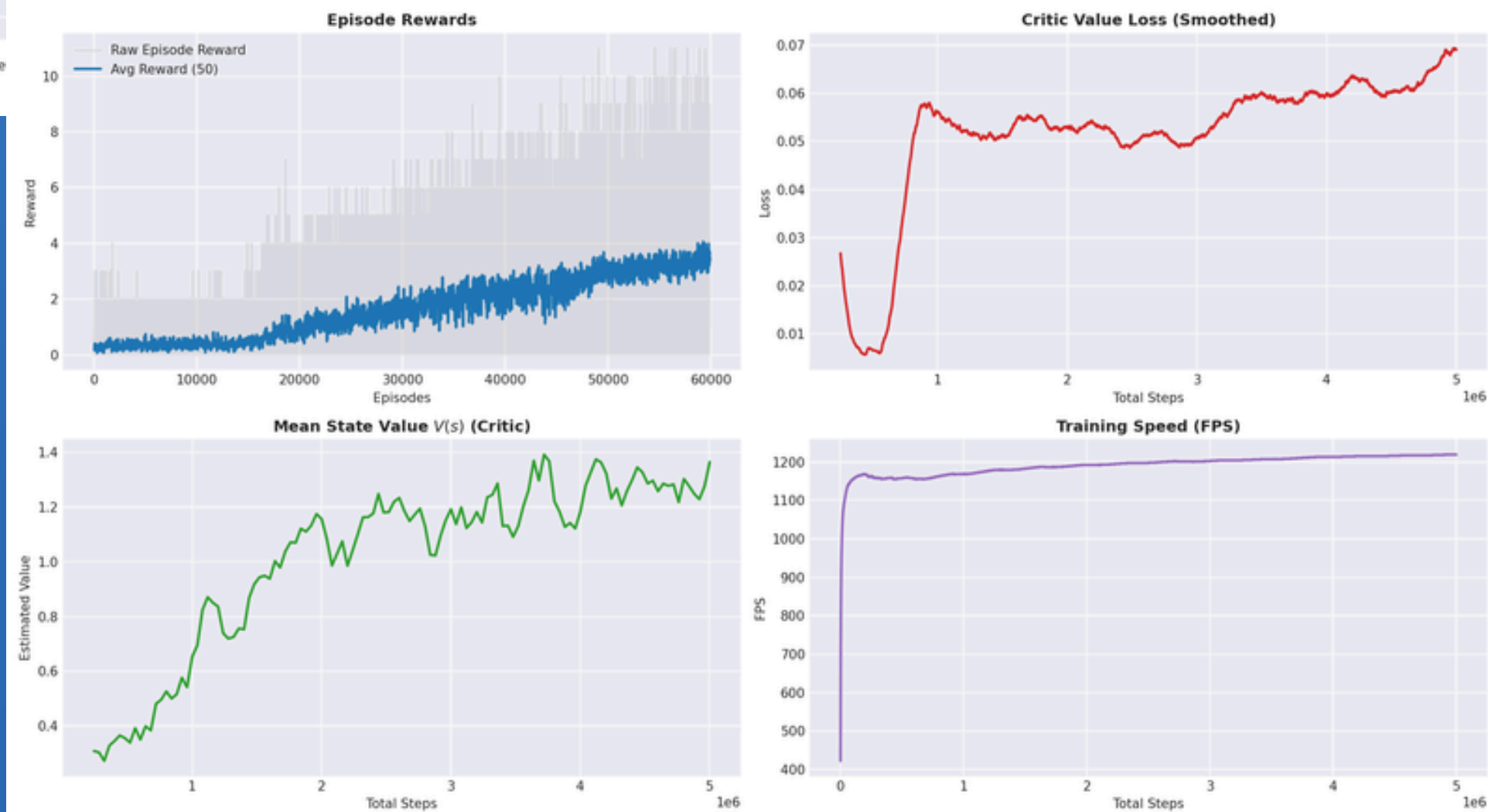
PPO Training Metrics: BreakoutNoFrameskip-v4
