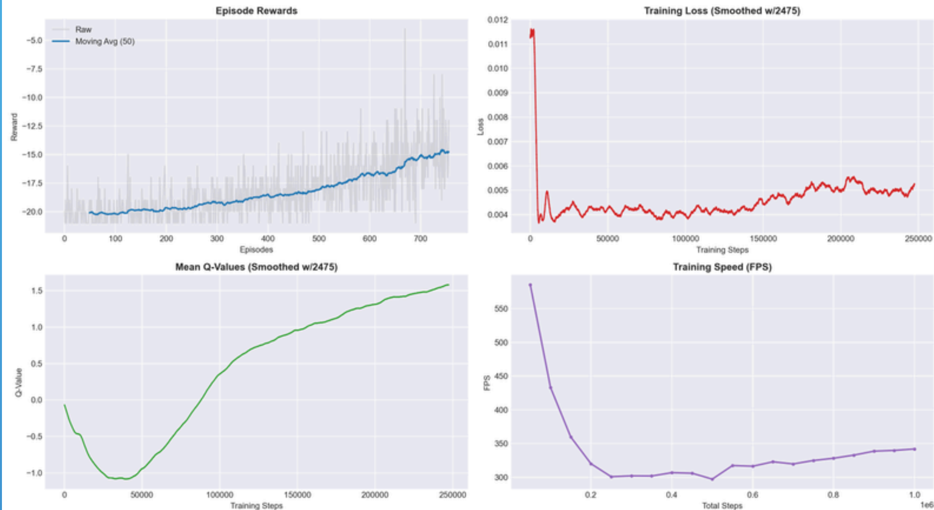
DQN Training Metrics: PongNoFrameskip-v4
