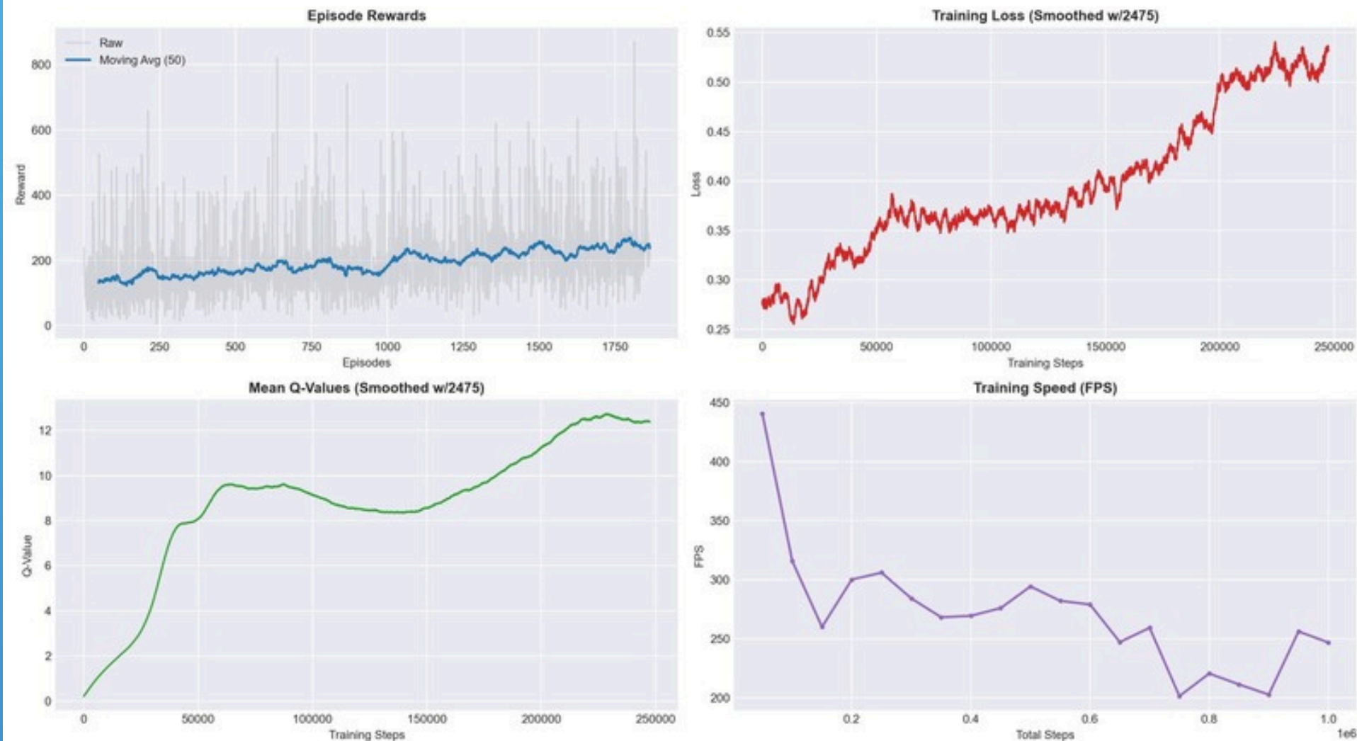
DQN Training Metrics: SpaceInvadersNoFrameskip-v4
