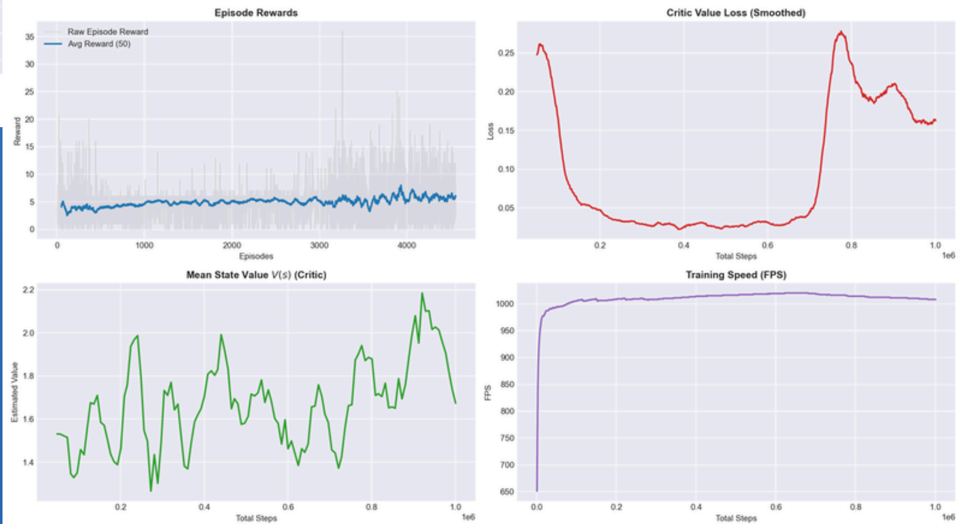
PPO Training Metrics: SpaceInvadersNoFrameskip-v4
