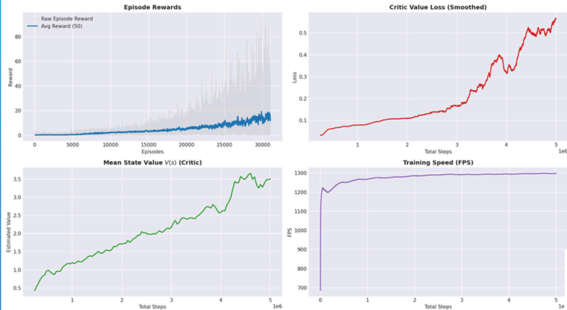
PPO Training Metrics: BreakoutNoFrameskip-v4
