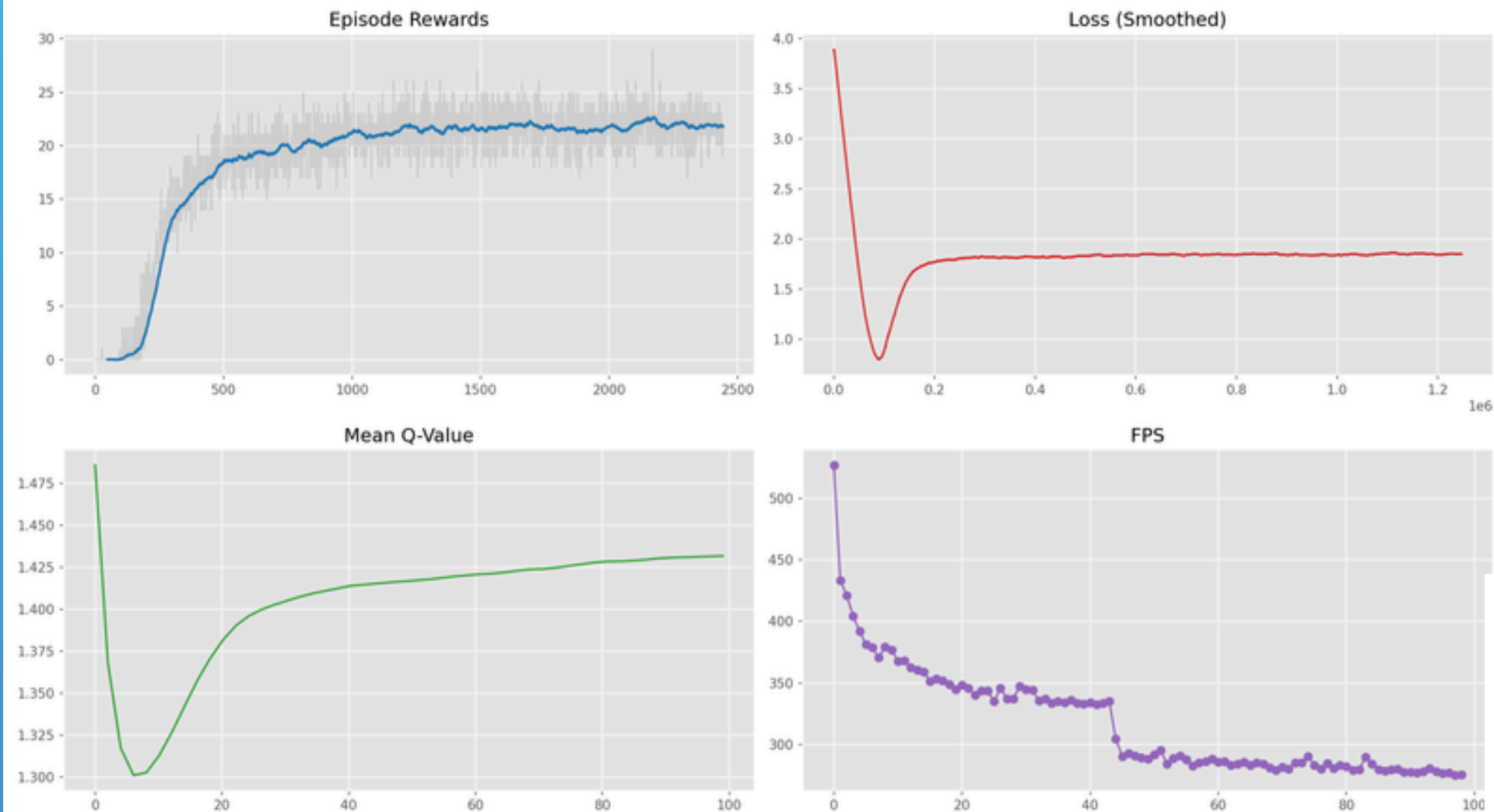
C51 Metrics - 1_Baseline
