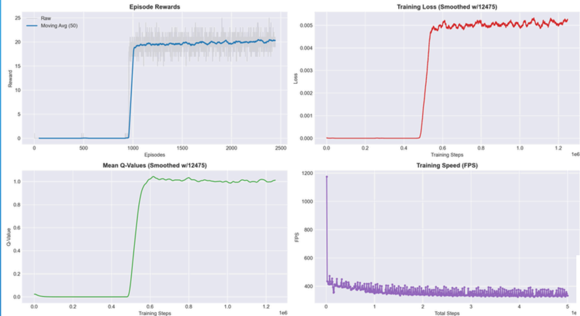
DQN Training Metrics: FreewayNoFrameskip-v4 (Duration: 3:51:52)
