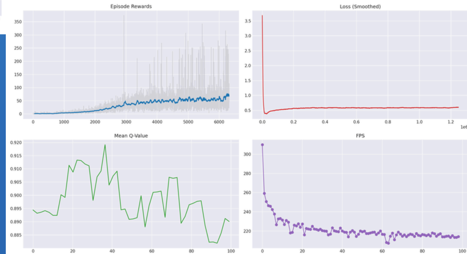
C51 Metrics - 3_Gamma_090
