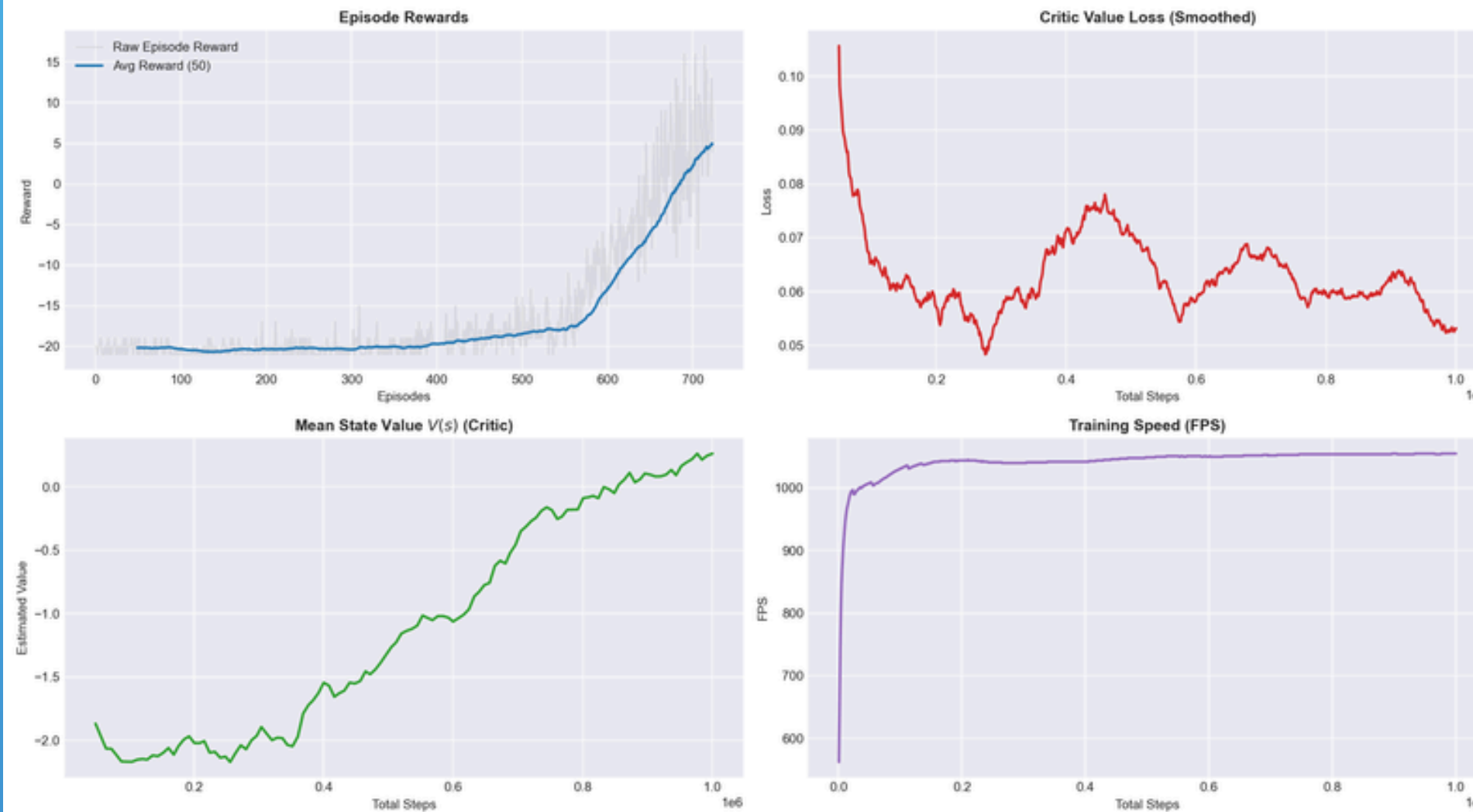
PPO Training Metrics: PongNoFrameskip-v4
