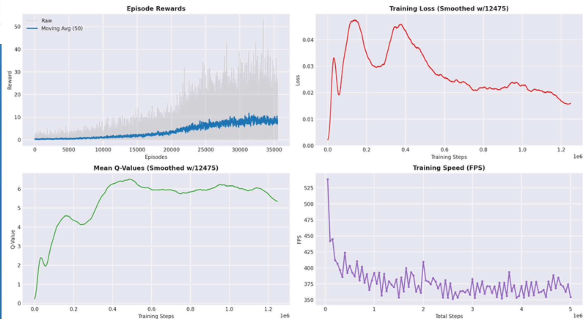
DQN Training Metrics: BreakoutNoFrameskip-v4
