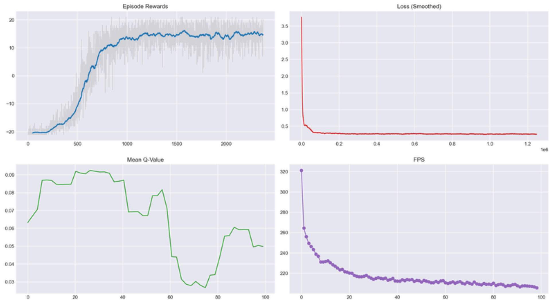
C51 Metrics - 3_Gamma_090
